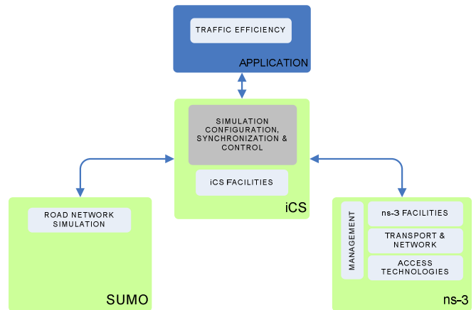
Figure 2: iTETRIS platform structure
